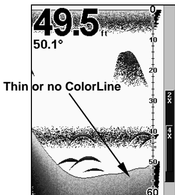
Little ColorLine (left) indicates a soft bottom, probably sand or mud. The wider ColorLine (right) indicates a harder, rocky bottom.
